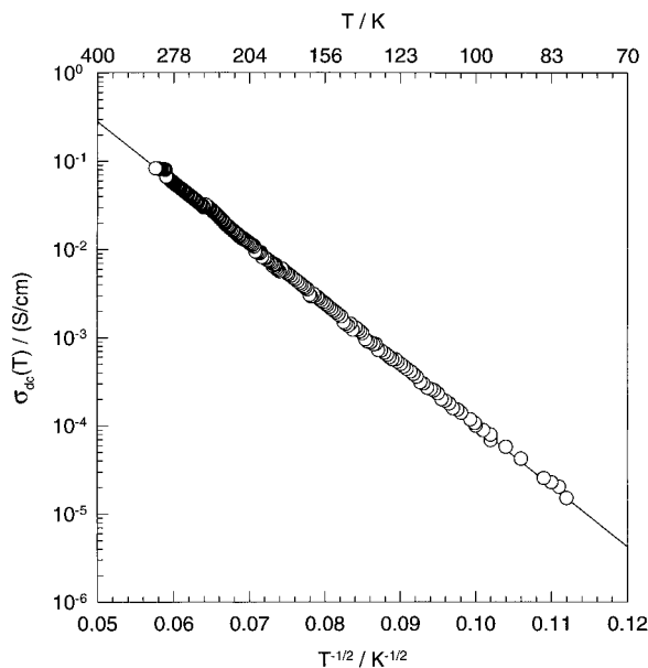
Figure 4. Temperature dependence of DC conductivity of LEB-SPAN sample plotted as \log \sigma vs T^{-1/2} (fit to the 1D-VRH model).
