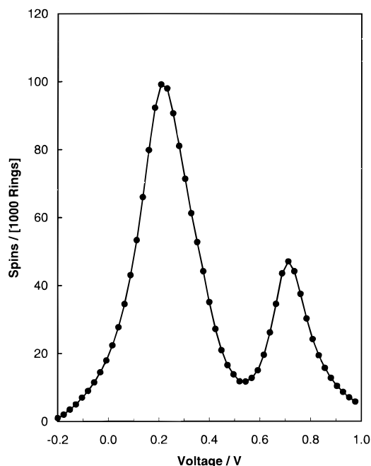
Figure 11. Simulation result of in situ EPR signal intensity as a function of CV scan potential. Dots are the computational data averaged for 500 hundred polymer chains of 1000 repeat units each.
