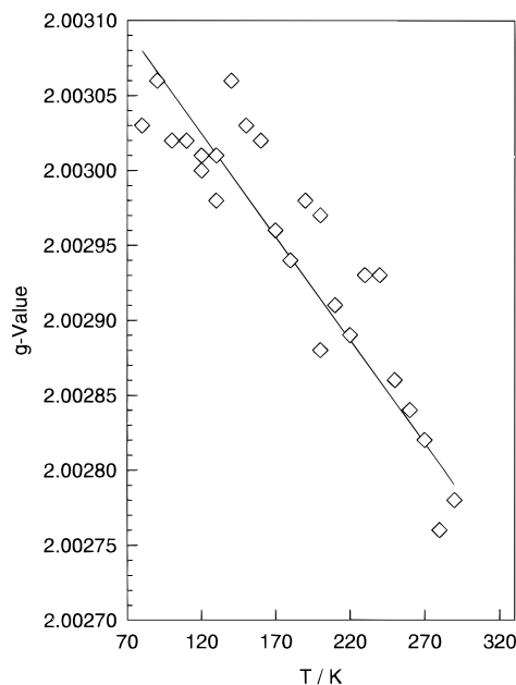
Figure 6. Temperature dependence of the g -value (measured at the magnetic field value that divides the spectral density in half) for LEB-SPAN sample ( \diamond ). The solid line is the linear fit to the data.
