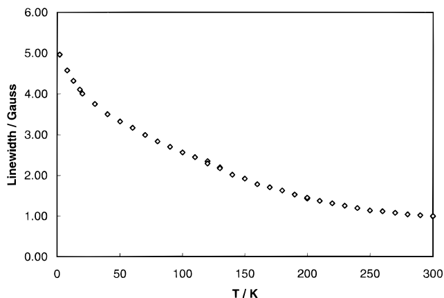
Figure 5. Temperature dependence of EPR linewidth for LEB-SPAN: full width at half maxima linewidth FWHM ( \diamond ).
