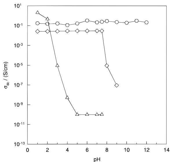
Figure 8. pH dependence of DC conductivity at room temperature for LEB-SPAN (○), EB-SPAN (◇), and PAN-HCl (△). The data of EB-SPAN and PAN-HCl were adapted from ref 3.
