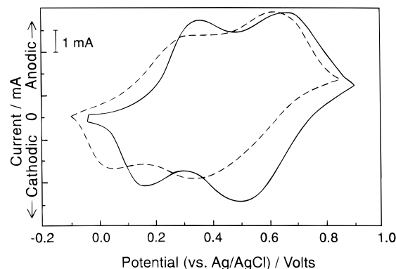
Figure 9. Cyclic voltammograms of LEB-SPAN in pH 1.0 (—) and 2.0 (---) buffer solutions. The scan rate is 50 mV/s and the current range is 100 mA.
