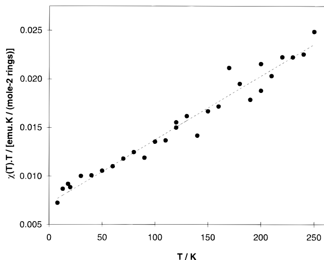
Figure 7. Magnetic susceptibility times temperature versus temperature plot. N(\epsilon_F) was obtained from the linear fit to the data (---) in the temperature region of (2 K, 250 K).
