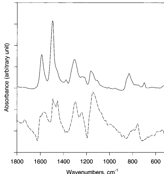
Figure 2. FTIR spectra: (—) EB in a KBr pellet; (---) ES in a KBr pellet.
