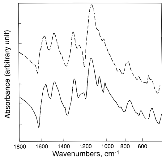
Figure 1. FTIR spectra: (—) self-doped form of LEB-SPAN in a KBr pellet; (---) self-doped form of EB-SPAN in a KBr pellet. The spectrum of EB-SPAN was adapted from ref 3.
