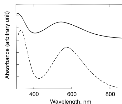
Figure 3. Solution UV–vis spectra for SPAN base: (—) LEB-SPAN in aqueous 0.1 M \text{NH}_4\text{OH} , maxima at 312 and 541 nm (eV); (---) EB-SPAN in aqueous 0.1 M \text{NH}_4\text{OH} , maxima at 320 and 563 nm. Cuvettes used for all of the above spectra are from Aldrich Chemical Co. (10-mm light path and transparent from 165 to 2600 nm). The spectrum of EB-SPAN was adapted from ref 3.
