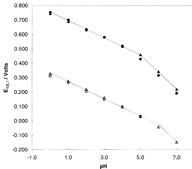
Figure 10. Half-wave potential, E_{1/2,i} , of LEB-SPAN sample vs pH plot: The first oxidation potential E_{1/2,1} as well as the second oxidation potential E_{1/2,2} was fit into two segments of straight lines (the slope of line from pH 1 to 5 is -59 \text{ mV/pH} while that from pH 5 to 7 is -118 \text{ mV/pH} ): (○ and ●) data for one electrode and (△ and ▲) data for another electrode. The electrodes were prepared with powders of the same batch of SPAN.
